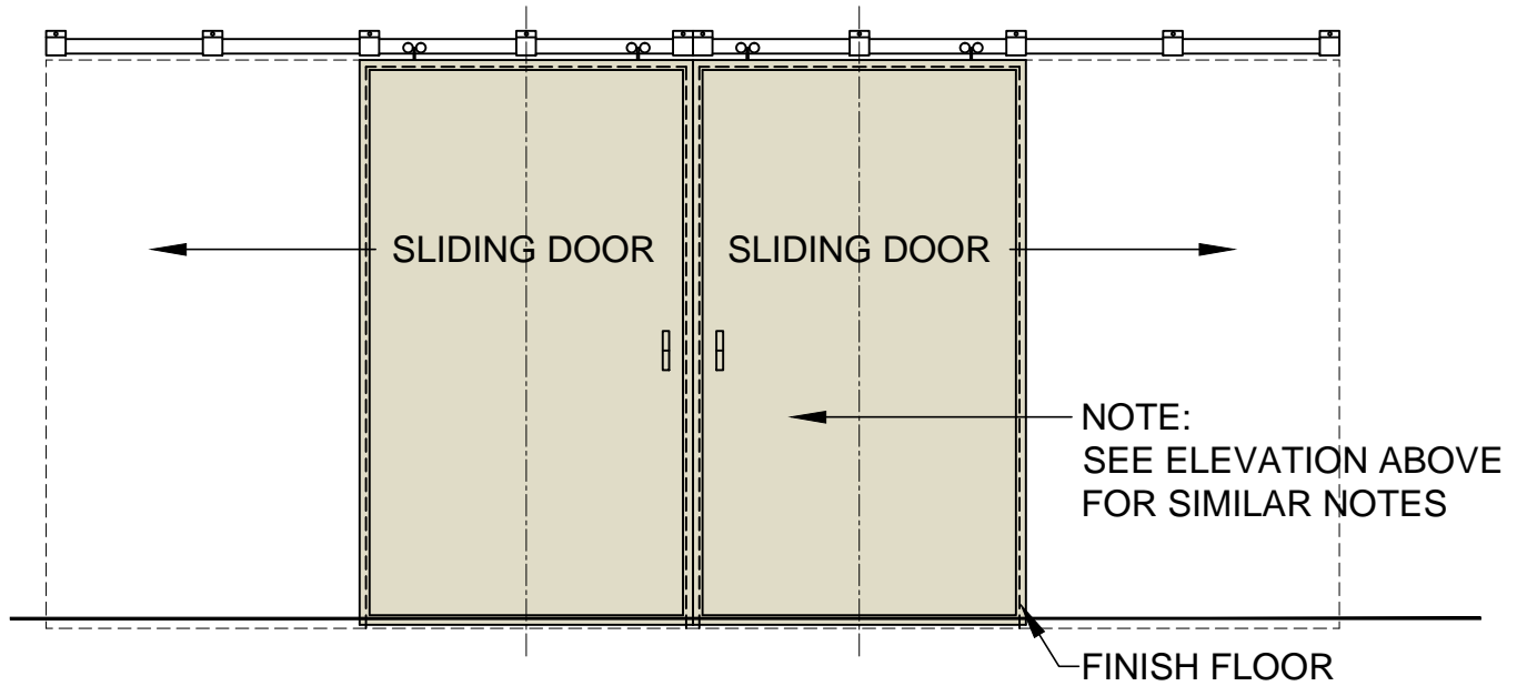
② RAY-BAR INDUSTRIAL LEAD LINED DOOR-DOUBLE 3/8"=1'-0"
